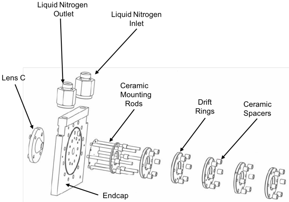
Figure 5. Breakdown of the drift cell endcap and components mounted on each side including: tapered exit lens (Lens C), copper drift rings, ceramic spacers, and liquid nitrogen inlet and outlet.
