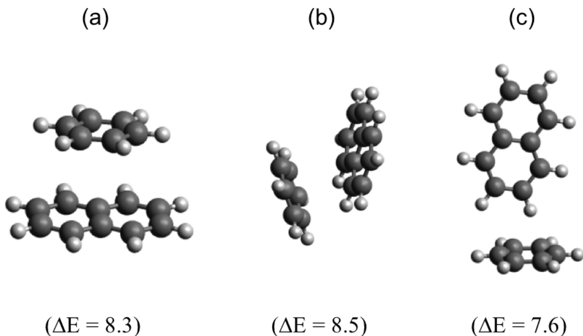
Figure 69. DFT structures and binding energies ( \Delta E , \text{kcal mol}^{-1} ) of the three classes of isomers for the naphthalene + (benzene) heterodimer: (a) stacked parallel, (b) V-shaped, (c) T-shaped calculated using the M11/cc-pVTZ where the lowest energy isomer is depicted.
