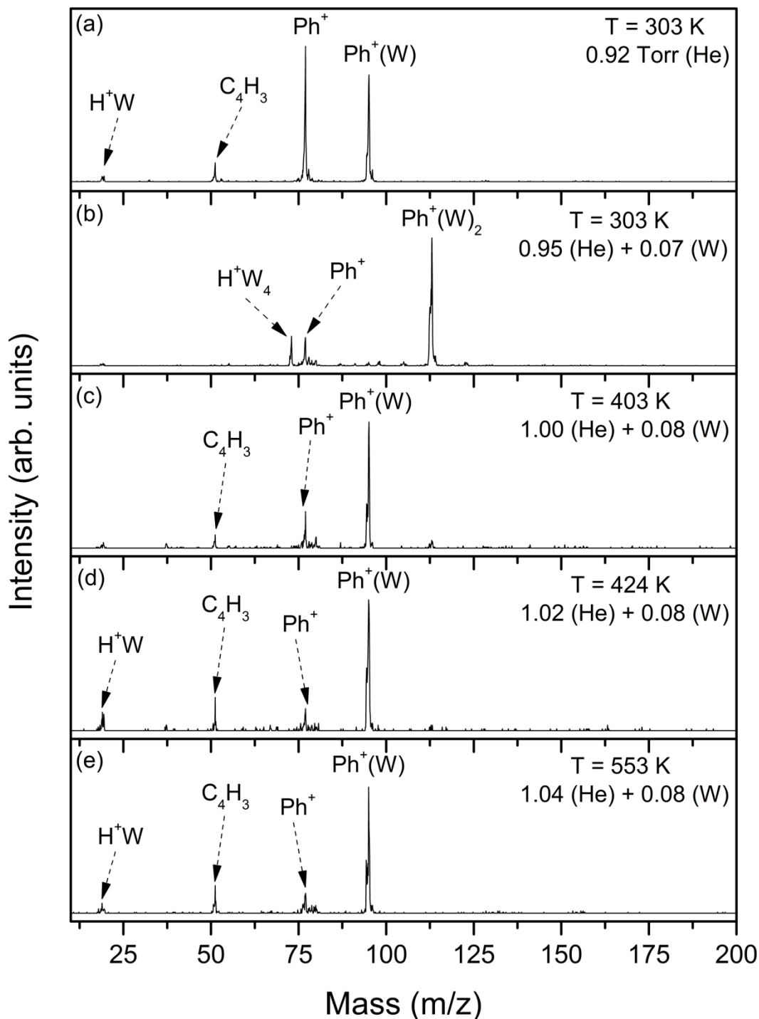
Figure 82. Mass spectra resulting from the injection of the mass-selected phenyl cation ( \text{C}_6\text{H}_5^+ , \text{Ph}^+ ) into He gas (a) or He/water (W) vapor mixture (b-e) at different pressures (Torr) and increasing temperatures (K) as indicated.
