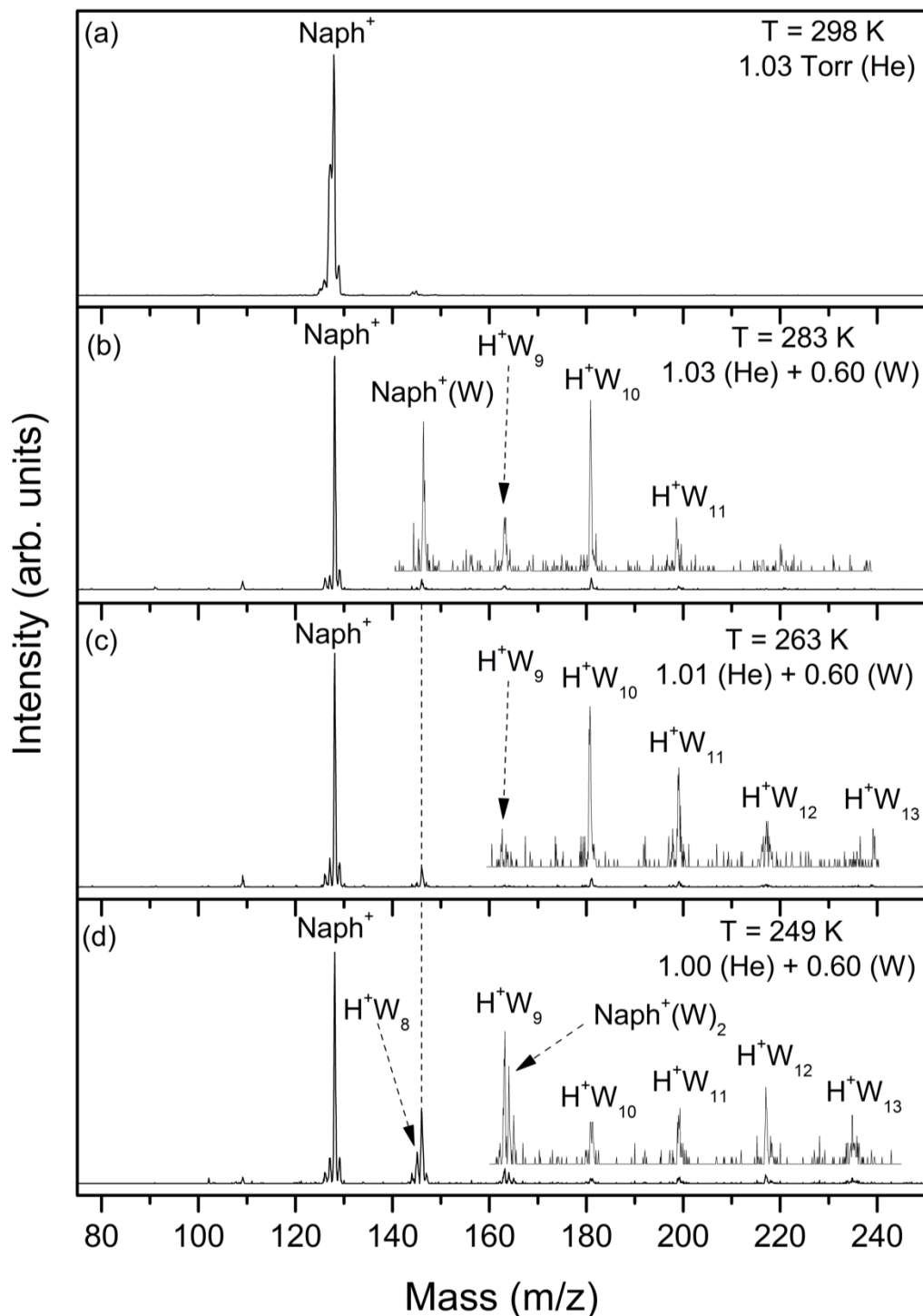
Figure 6. Mass spectra obtained resulting from the injection of the mass-selected naphthalene radical cation ( \text{C}_{10}\text{H}_8^{+\cdot} , \text{Naph}^+ ) into He gas (a) or He/water ( \text{H}_2\text{O} , W) vapor mixture (b-d) at different pressures (Torr) and temperatures (K) as indicated.
