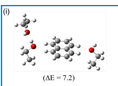
Figure 29. DFT Structures and binding energies ( \Delta E , kcal mol -1 , calculated according to Equation 4.3) for higher energy isomers of the C 10 H 8 •+ (EtOH) n clusters for n = 1-3 obtained at the B3LYP/6-311++G** level.
