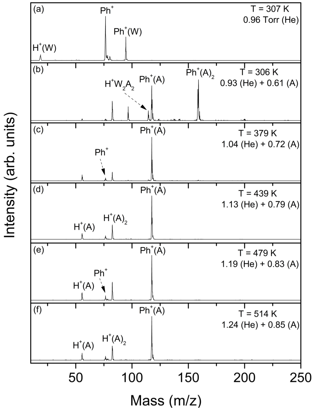
Figure 94. Mass spectra resulting from the injection of the mass-selected phenyl cation ( \text{C}_6\text{H}_5^+ , \text{Ph}^+ ) into \text{He} gas (a) or \text{He}/\text{acetone nitrile} ( \text{CH}_3\text{CN} , A) gas mixture (b-f) at different pressures (Torr) and increasing temperatures (K) as indicated.
