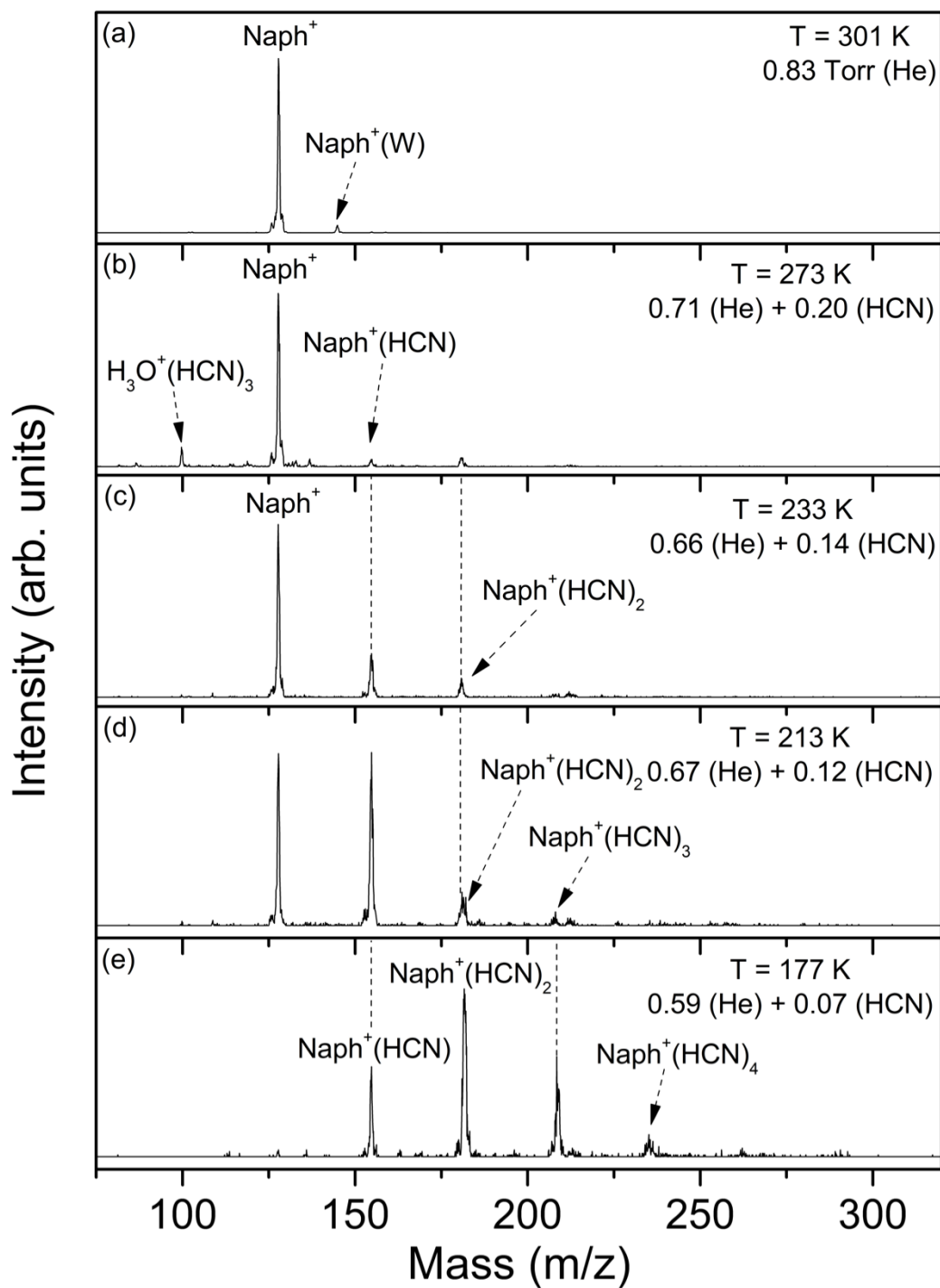
Figure 38. Mass spectra resulting from the injection of the mass-selected naphthalene radical cation ( C_{10}H_8^+ , Naph^+ ) into He gas (a) or He/HCN vapor mixture (b-e) at different pressures (Torr) and decreasing temperatures (K) as indicated.
