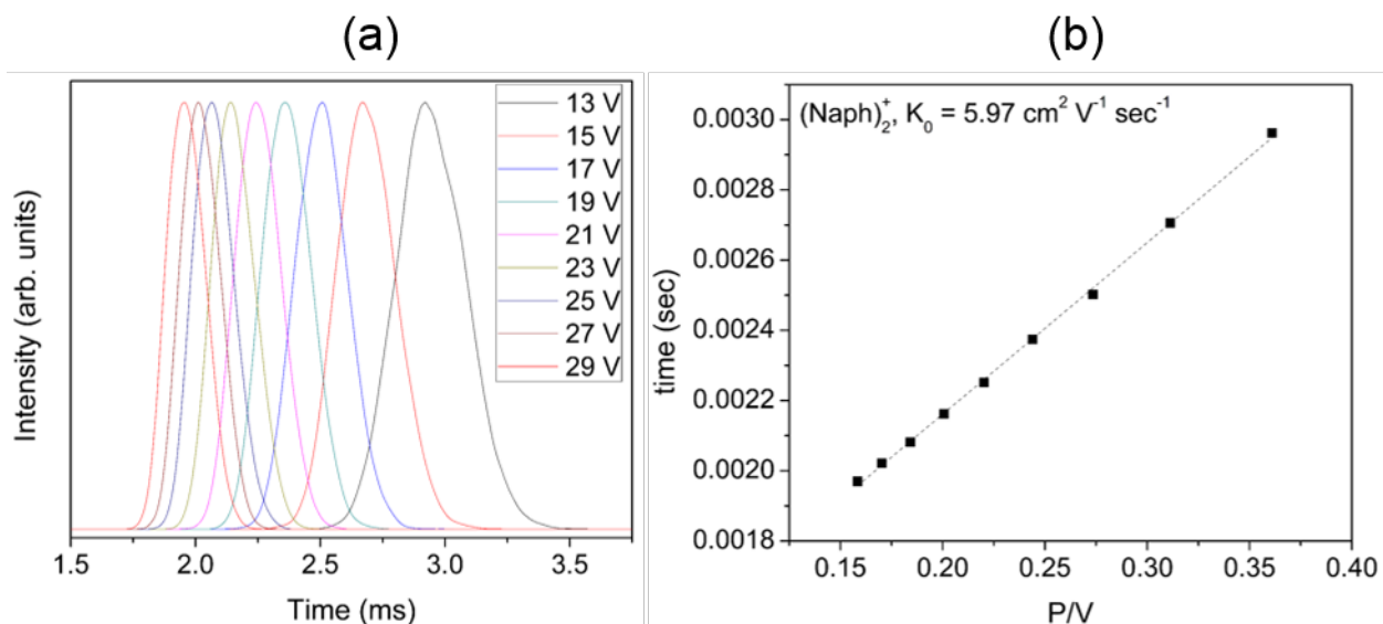
Figure 63. (a) ATDs and (b) t_d versus P/V plot for the naphthalene radical cation homodimer (\text{Naph})_2^+ . All the data are obtained in 4.5 Torr helium at a temperature of 302 K.
