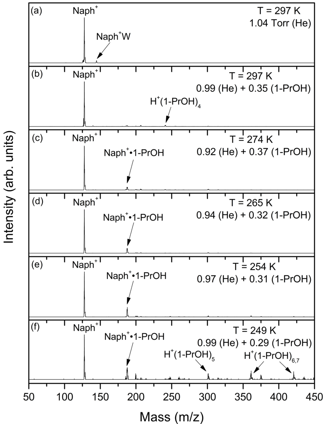
Figure 20. Mass spectra resulting from the injection of the mass-selected naphthalene radical cations ( \text{C}_{10}\text{H}_8^{+\bullet} , \text{Naph}^+ ) into He gas (a) or He/1-propanol (1-PrOH) vapor mixture (b-f) at different pressures (Torr) and temperatures (K) as indicated.
