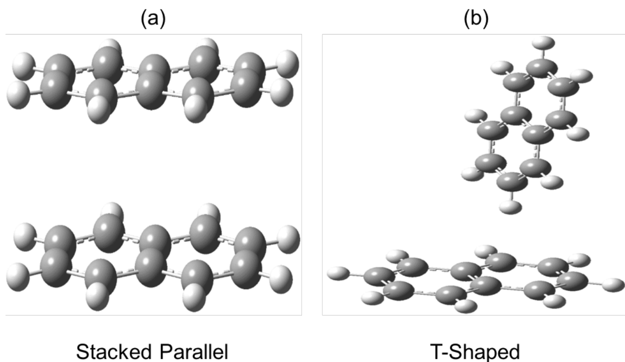
Figure 64. Two classes of isomers for the naphthalene radical cation homodimers: (a) stacked parallel and (b) T-shaped. The structures are optimized at the B3LYP/6-311++G** level of theory.
