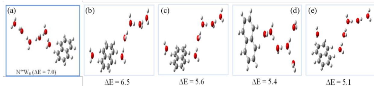
Figure 13. DFT structures and binding energies ( \Delta E , kcal mol -1 , calculated using Equation 4.3) for (a) the lowest energy isomer of the C_{10}H_8^{+\bullet}(H_2O)_6 cluster and (b-d) higher energy isomers with corresponding binding energies.
