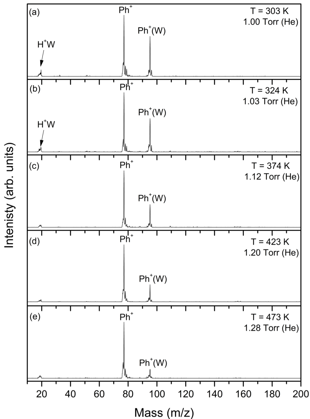
Figure 81. Mass spectra resulting from the injection of the mass-selected phenyl cation ( \text{C}_6\text{H}_5^+ , \text{Ph}^+ ) into He gas at different pressures and temperatures as indicated.
