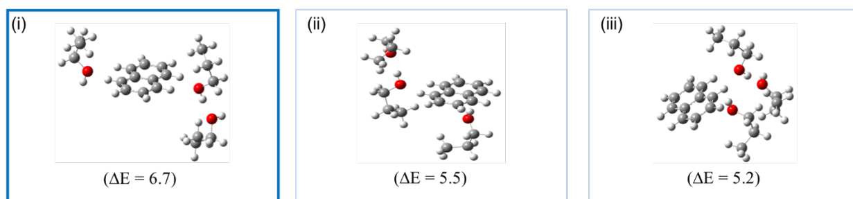
Figure 31. DFT Structures and binding energies ( \Delta E , kcal mol -1 , calculated according to Equation 4.3) for higher energy isomers of the C_{10}H_8^{++}(1-PrOH)_n clusters for n = 1-3 obtained at the B3LYP/6-311++G** level.
