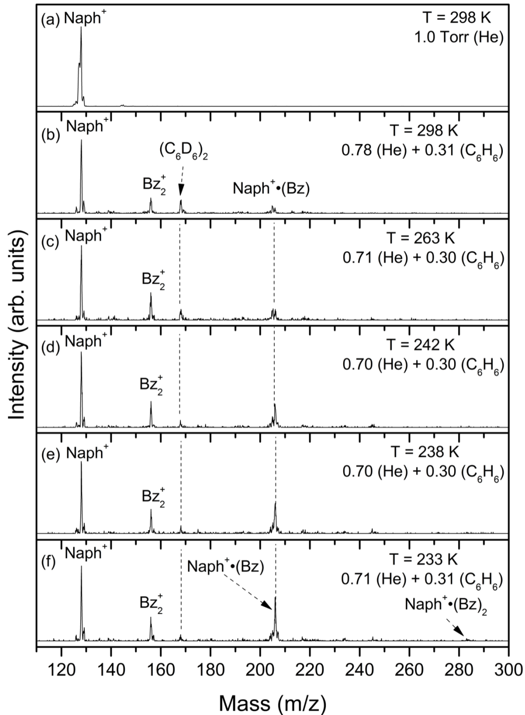
Figure 66. Mass spectra resulting from the injection of the mass-selected naphthalene radical cation ( \text{C}_{10}\text{H}_8^+ , \text{Naph}^+ ) into the drift cell containing He gas (a) or He/benzene ( \text{C}_6\text{H}_6 ) vapor mixture (b-f) at different temperatures and pressures as indicated.
