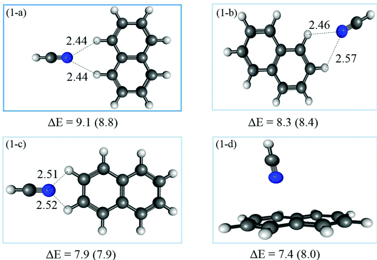
Figure 41. Structures of the four lowest energy isomers of the C_{10}H_8^{++}(HCN) complex obtained using two functionals: M06-2X and \omega 97X-D, within the 6-311+G** basis set. The calculated energies \Delta E in \text{kcal mol}^{-1} are given using M06-2X and \omega 97X-D (in parenthesis) methods.
