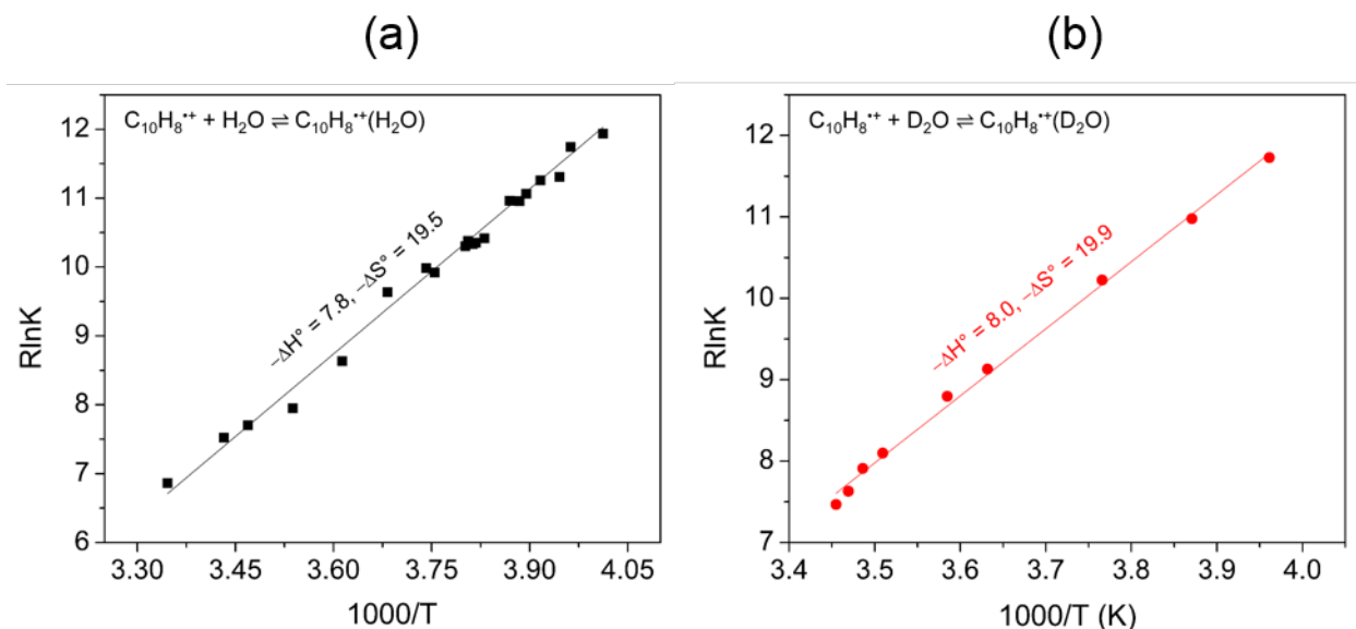
Figure 7. van't Hoff plots for the temperature dependence of the equilibrium constants of the association reaction of naphthalene radical cation with water where H 2 O is shown in (a) and D 2 O shown in (b). The resulting -\Delta H^\circ and -\Delta S^\circ are in (kcal mol -1 ) and (cal mol -1 K -1 ) respectively. The error for the measurements are \pm 1 kcal mol -1 for -\Delta H^\circ and \pm 2 cal mol -1 K -1 for -\Delta S^\circ .
