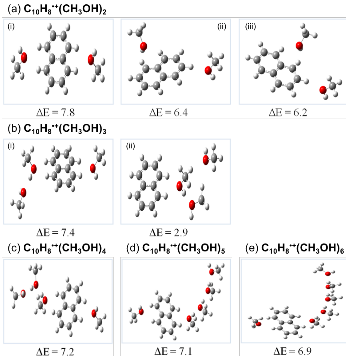
Figure 17. DFT Structures and binding energies ( \Delta E , kcal mol -1 , calculated using Equation 4.3) for higher energy isomers of the C_{10}H_8^{++}(CH_3OH)_n clusters for n = 2-6 obtained at the B3LYP/6-311++G** level.
