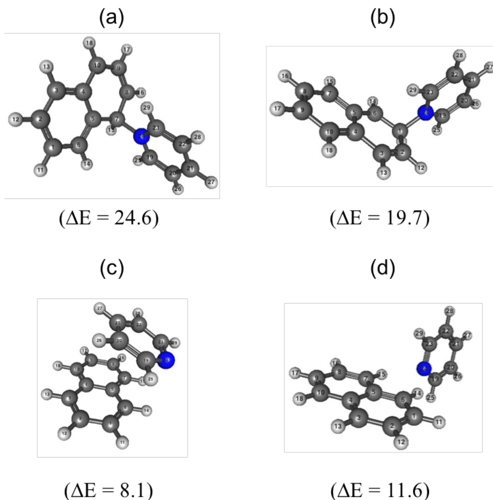
Figure 79. DFT structures and binding energies ( \Delta E , kcal mol -1 ) of four isomers for the naphthalene •+ (pyridine) heterodimer: (a) covalent structure 1 (C1), (b) covalent structure 2 (C2), (c) stacked parallel, and (d) T-shaped calculated at the M06-2X/cc-pVTZ level of theory.
