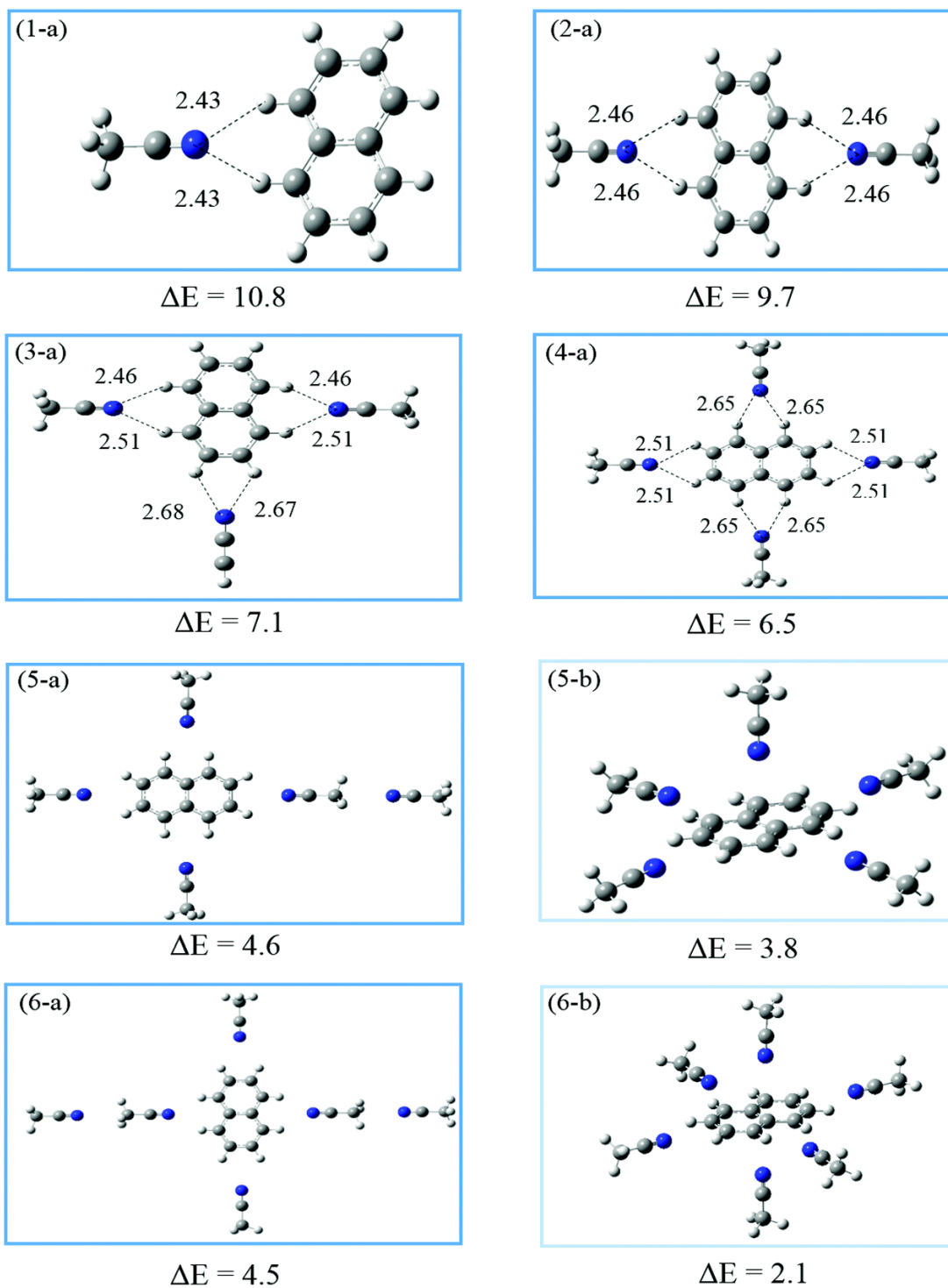
Figure 49. Structures of the lowest energy isomers of the C_{10}H_8^+(CH_3CN)_n clusters for n = 1-4 and the two lowest energy isomers for n = 5 and 6 obtained using the B3LYP method within the 6-311++G** basis set. The calculated energies \Delta E are given in \text{kcal mol}^{-1}
