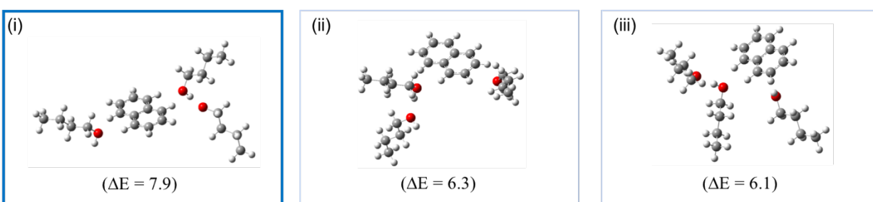
Figure 35. DFT Structures and binding energies ( \Delta E , kcal mol -1 , calculated according to Equation 4.3) for higher energy isomers of the C_{10}H_8^{*+}(1-BuOH)_n clusters for n = 1-3 obtained at the B3LYP/6-311++G** level.
