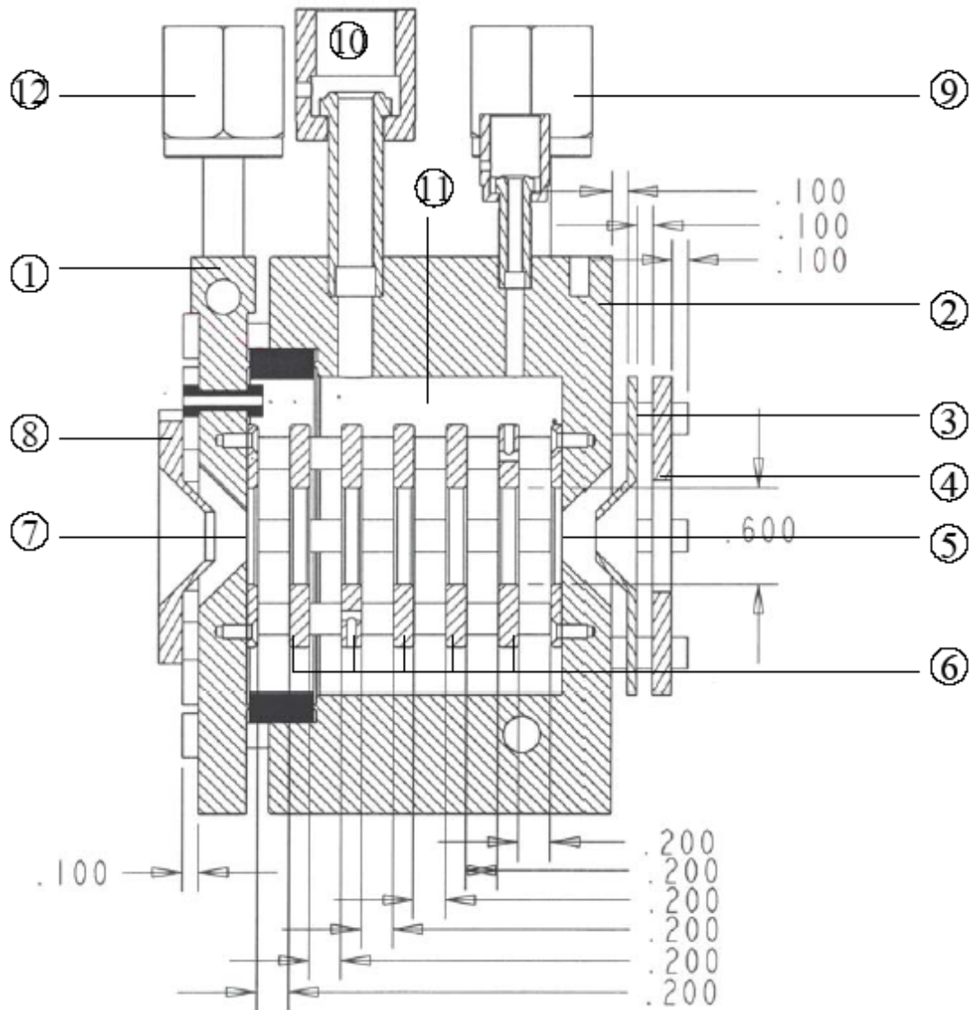
Figure 4. Side view cross section of the drift cell used in the VCU QMS-IM-QMS system with the following components (all units in inches): (1) Endcap, (2) Reaction Cell Body, (3) Entrance Lens (Lens B), Tapered Entrance Lens (Lens A), (5) Entrance Orifice (0.25 mm), (6) Drift Rings (inside of drift cell body), (7) Exit Orifice (0.25 mm), (8) Tapered Exit Lens (Lens C), (9) Cell Body Liquid Nitrogen Inlet, (10) Baratron Connection, (11) Drift Cell, (12) Endcap Liquid Nitrogen Inlet.
