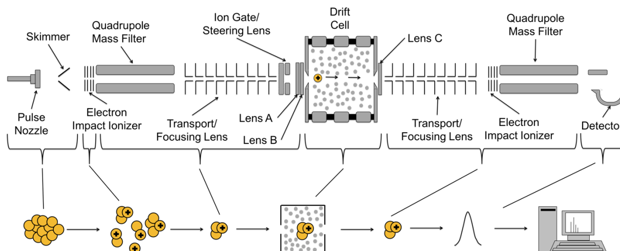
Figure 2. General diagram for the experimental setup of the VCU QMS-IM-QMS system. 87
