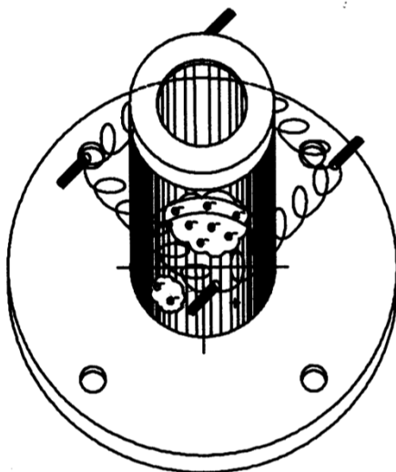
Figure 3. Schematic drawing of the ion region basket surrounded by the tungsten filament illustrating the region where ionization occurs.
