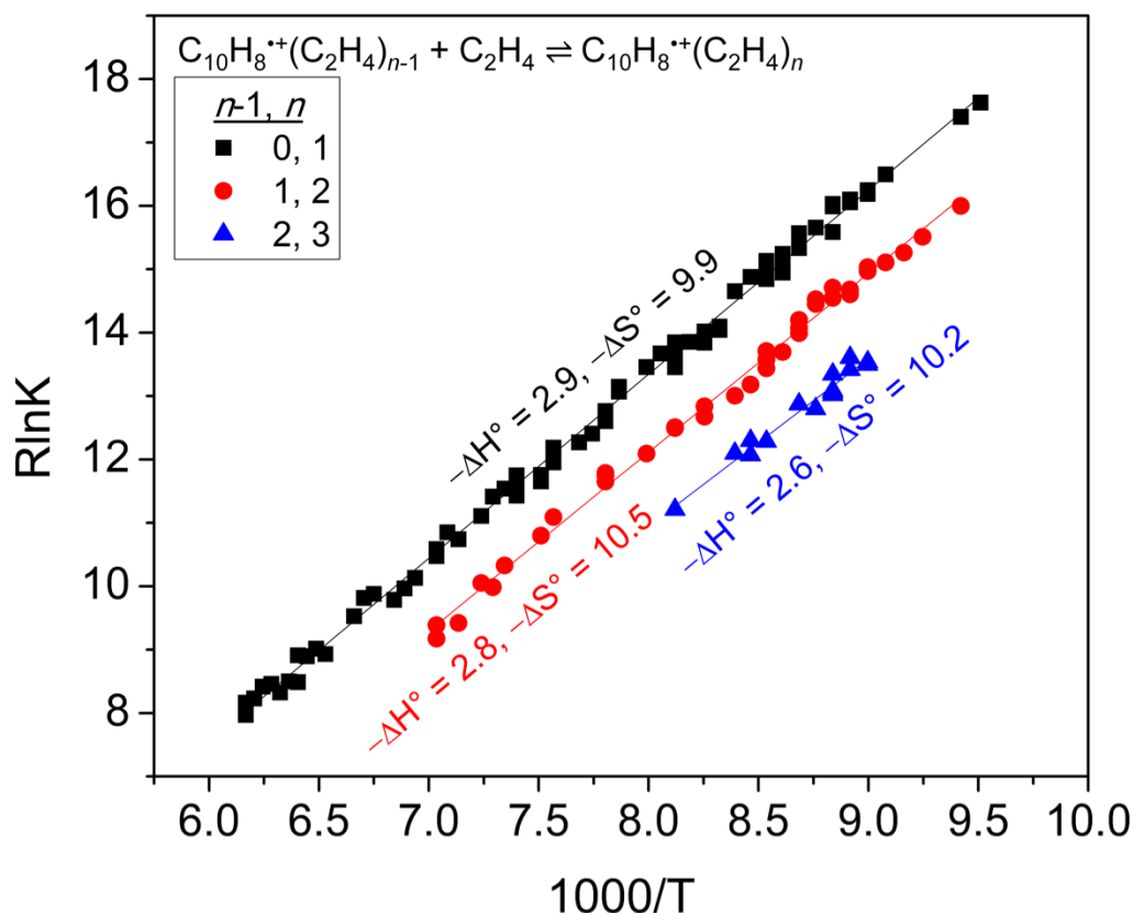
Figure 56. van't Hoff plots for the temperature dependence of the equilibrium constants of the association reaction of naphthalene radical cation with ethylene for the first three solvation steps. The resulting \Delta H^\circ and \Delta S^\circ are in ( \text{kcal mol}^{-1} ) and ( \text{cal mol}^{-1} \text{K}^{-1} ) respectively. The error for the measurements are \pm 1 \text{ kcal mol}^{-1} for -\Delta H^\circ and \pm 2 \text{ cal mol}^{-1} \text{K}^{-1} for -\Delta S^\circ .
