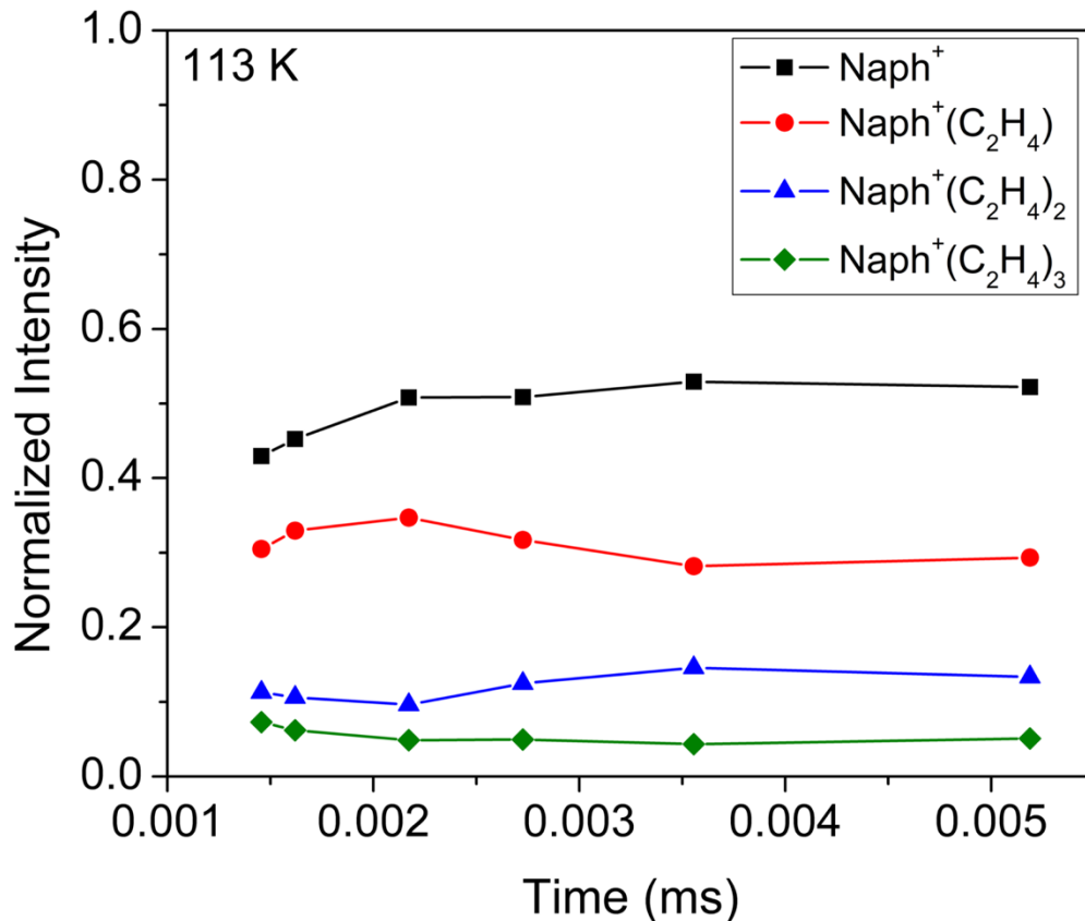
Figure 57. Time profile based on the arrival time distributions (ATDs) of the naphthalene radical cation ( \text{Naph}^+ ) and the first three association products with ethylene, \text{C}_{10}\text{H}_8^{*+}(\text{C}_2\text{H}_4)_n for n = 1-3 ( \text{Naph}^+(\text{C}_2\text{H}_4)_n for n = 1-3 ), obtained following the injection of the mass-selected naphthalene radical cation into \text{He}/\text{C}_2\text{H}_4 gas mixtures at 113 K.
