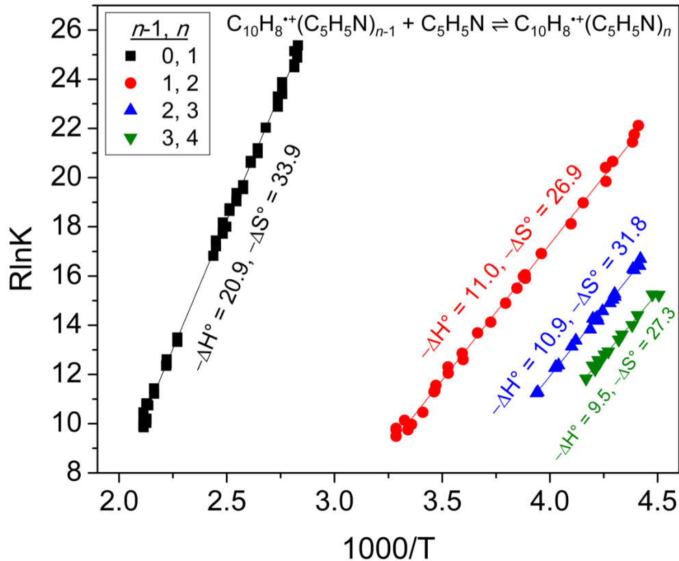
Figure 74. van't Hoff plots for the temperature dependence of the equilibrium constants of the association reaction of naphthalene radical cation with pyridine for the first four solvation steps. The resulting \Delta H^\circ and \Delta S^\circ are in ( \text{kcal mol}^{-1} ) and ( \text{cal mol}^{-1} \text{K}^{-1} ) respectively. The error for the measurements are \pm 1 \text{ kcal mol}^{-1} for -\Delta H^\circ and \pm 2 \text{ cal mol}^{-1} \text{K}^{-1} for -\Delta S^\circ .
