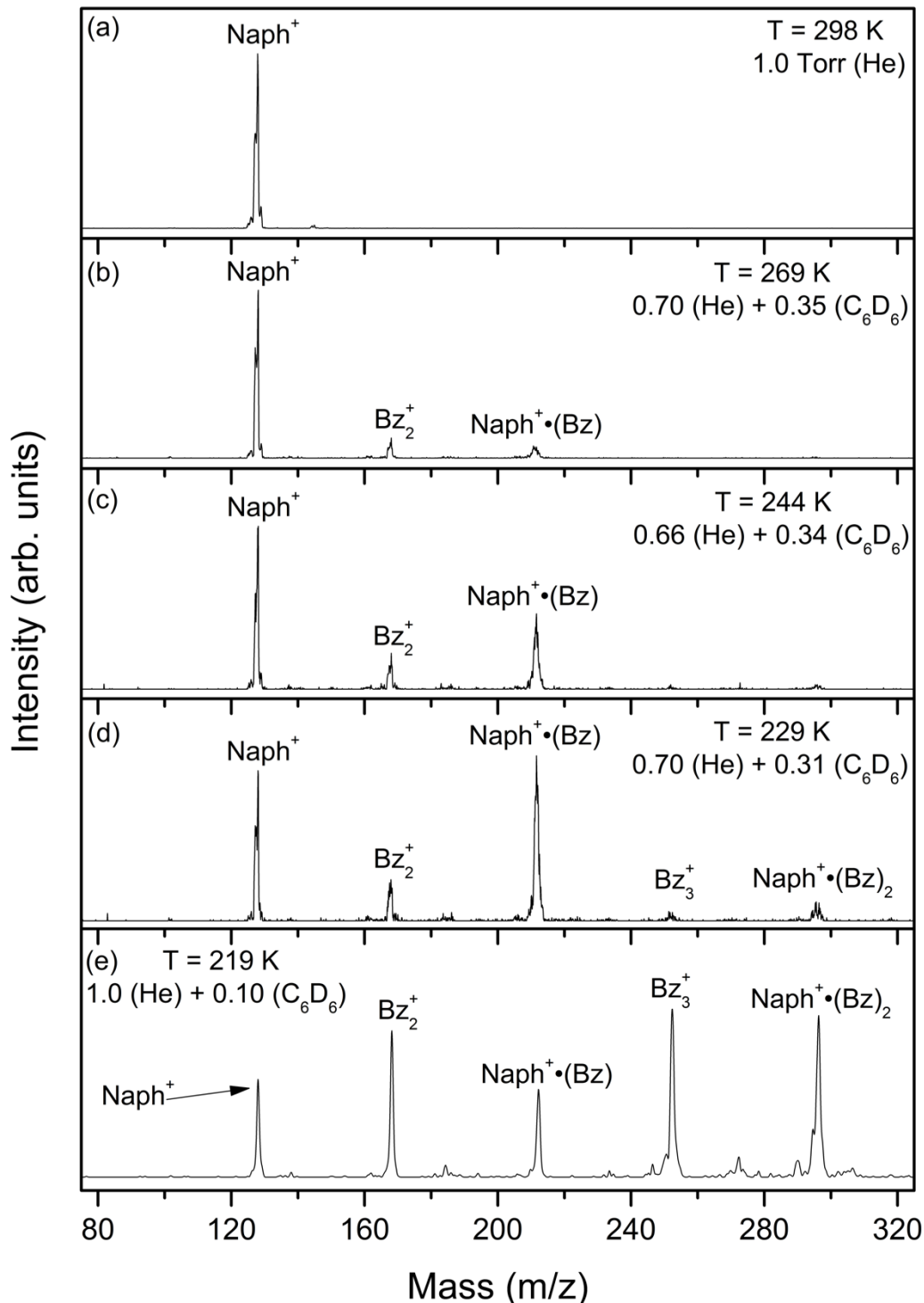
Figure 65. Mass spectra resulting from the injection of the mass-selected naphthalene radical cation ( \text{C}_{10}\text{H}_8^{+\cdot} , \text{Naph}^+ ) into the drift cell containing He gas (a) or He/benzene ( \text{C}_6\text{D}_6 ) vapor mixture (b-e) at different temperatures and pressures as indicated.
