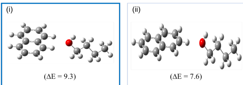
(b) C_{10}H_8^{*+}(1-BuOH)_2
