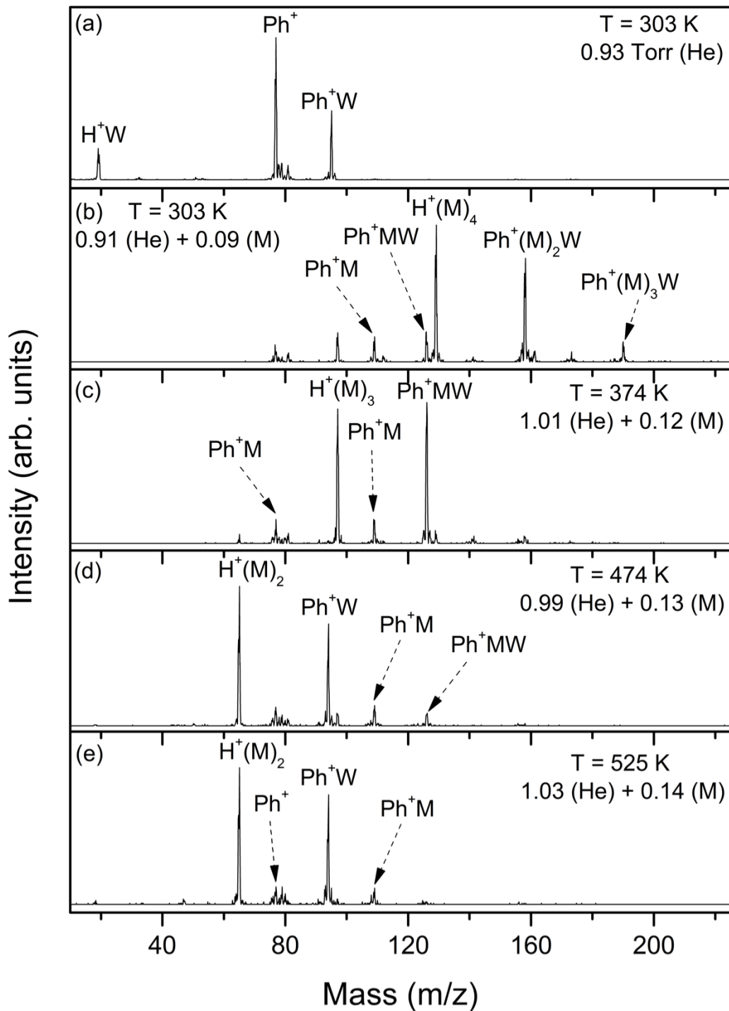
Figure 89. Mass spectra resulting from the injection of the mass-selected phenyl cation ( \text{C}_6\text{H}_5^+ , \text{Ph}^+ ) into He gas (a) or He/methanol (M) vapor mixture (b-e) at different pressures (Torr) and increasing temperatures (K) as indicated.
