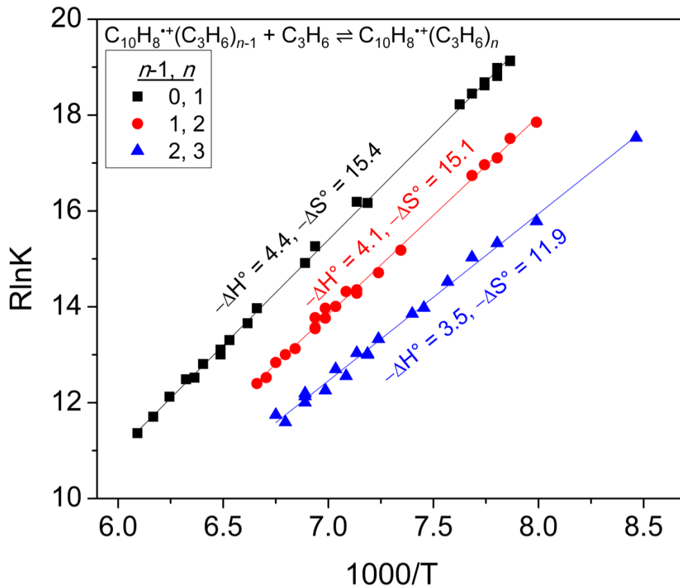
Figure 58. van't Hoff plots for the temperature dependence of the equilibrium constants of the association reaction of naphthalene radical cation with propylene for the first three solvation steps. The resulting \Delta H^\circ and \Delta S^\circ are in (kcal mol -1 ) and (cal mol -1 K -1 ) respectively. The error for the measurements are \pm 1 kcal mol -1 for -\Delta H^\circ and \pm 2 cal mol -1 K -1 for -\Delta S^\circ .
