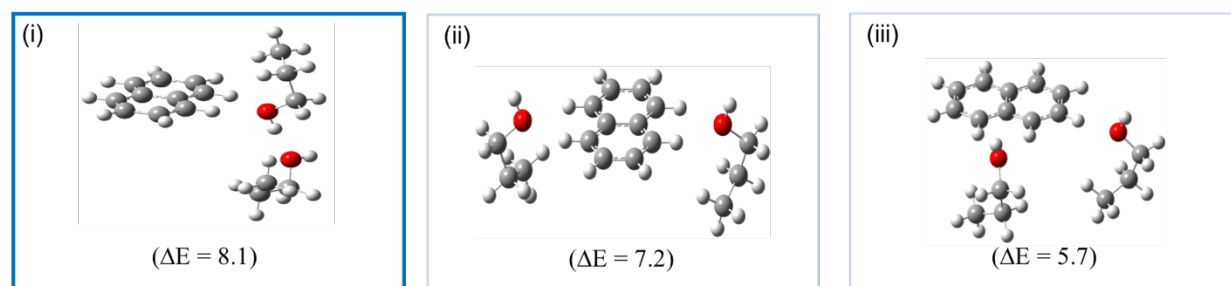
(c) C_{10}H_8^{++}(1-PrOH)_3
