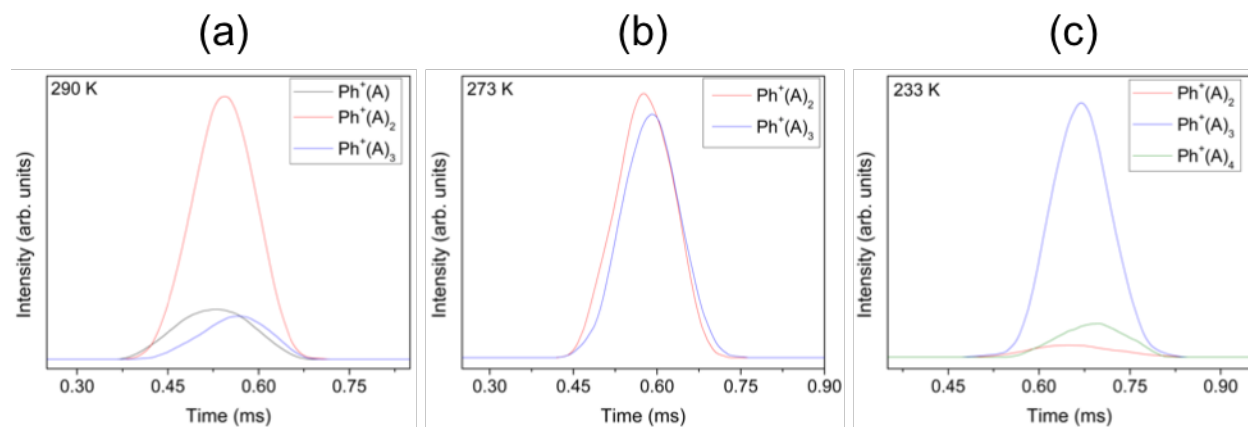
Figure 97. Arrival time distributions (ATDs) of the first four association products of the phenyl cation with acetonitrile (A), C_6H_5^+(CH_3CN)_n for n = 1-4 ( Ph^+(A)_n , n = 1-4 ), obtained following the injection of the mass-selected phenyl cation into He/ CH_3CN vapor mixtures at: (a) 290 K, (b) 273 K, and (c) 233 K. Similar ATD overlap suggests the reaction is in equilibrium.
