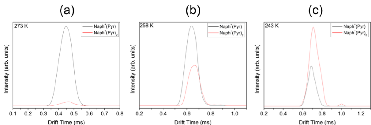
Figure 76. Arrival time distributions (ATDs) of the naphthalene + (pyridine) heterodimer, \text{C}_{10}\text{H}_8^+(\text{C}_5\text{H}_5\text{N}) ( \text{Naph}^+(\text{Pyr}) ), and the second association product, \text{C}_{10}\text{H}_8^{++}(\text{C}_5\text{H}_5\text{N})_2 ( \text{Naph}^+(\text{Pyr})_2 ), obtained following the injection of the mass-selected naphthalene radical cation into He/ \text{C}_5\text{H}_5\text{N} vapor mixture at: (a) 273 K, (b) 258 K, and 243 K. Similar ATD overlap suggests the reaction is in equilibrium.
