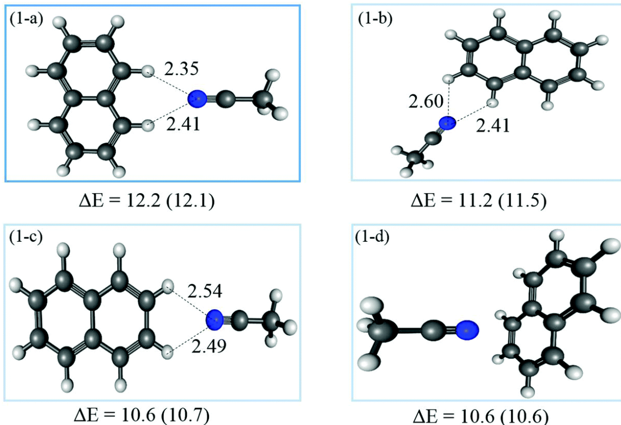
Figure 47. Structures of the four lowest energy isomers of the C_{10}H_8^{++}(CH_3CN) complex obtained using two functionals: M06-2X and \omega 97X-D, within the 6-311+G** basis set. The calculated energies \Delta E in \text{kcal mol}^{-1} are given using M06-2X and \omega 97X-D (in parenthesis) methods.
