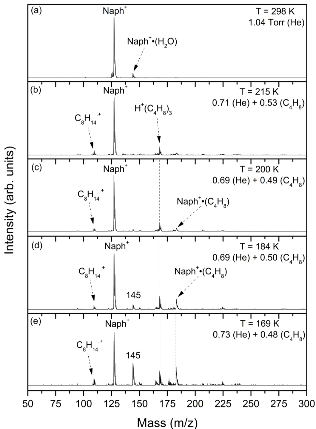
Figure 55. Mass spectra resulting from the injection of the mass-selected naphthalene radical cation ( C_{10}H_8^+ , Naph^+ ) into He gas (a) or He/isobutene ( C_4H_8 ) gas mixture (b-f) at different pressures (Torr) and temperatures (K) as indicated.
