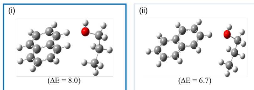
(b) C_{10}H_8^{++}(1-PrOH)_2
