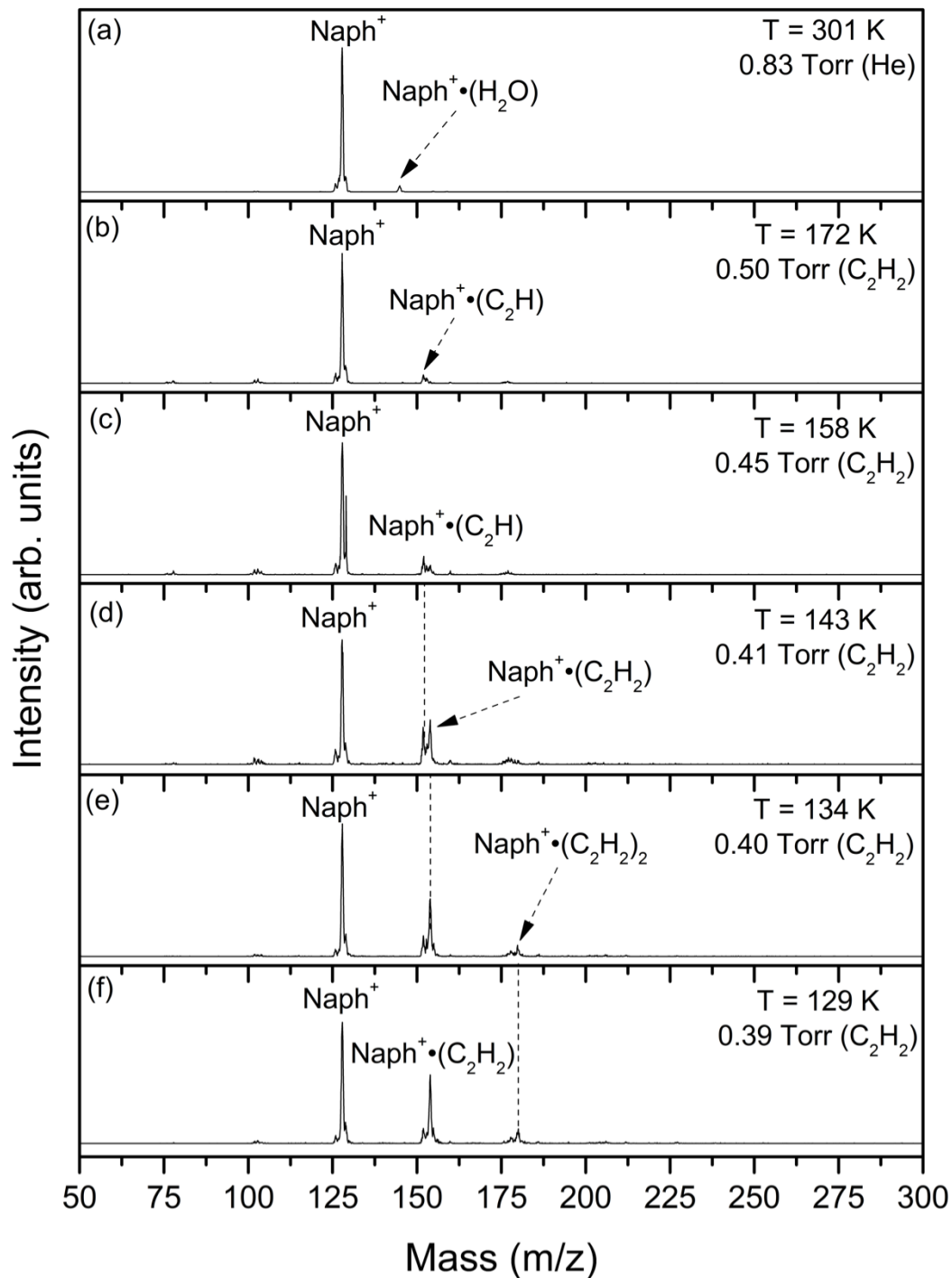
Figure 50. Mass spectra resulting from the injection of the mass-selected naphthalene radical cation ( \text{C}_{10}\text{H}_8^{+\bullet} , \text{Naph}^+ ) into He gas (a) or acetylene ( \text{C}_2\text{H}_2 ) gas (b-f) at different pressures (Torr) and temperatures (K) as indicated.
