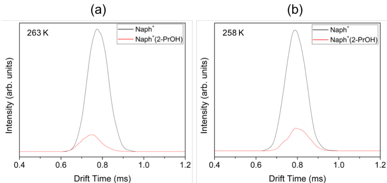
Figure 27. Arrival time distributions (ATDs) of the naphthalene radical cation ( \text{Naph}^{\bullet+} ) and the first association product with 2-propanol, \text{C}_{10}\text{H}_8^{\bullet+}(\text{2-PrOH}) ( \text{Naph}^{\bullet+}(\text{2-PrOH}) ), obtained following the injection of the mass-selected naphthalene radical cation into He/2-PrOH vapor mixture at: (a) 263 K and (b) 258 K. Similar ATD overlap suggests the reaction is in equilibrium.
