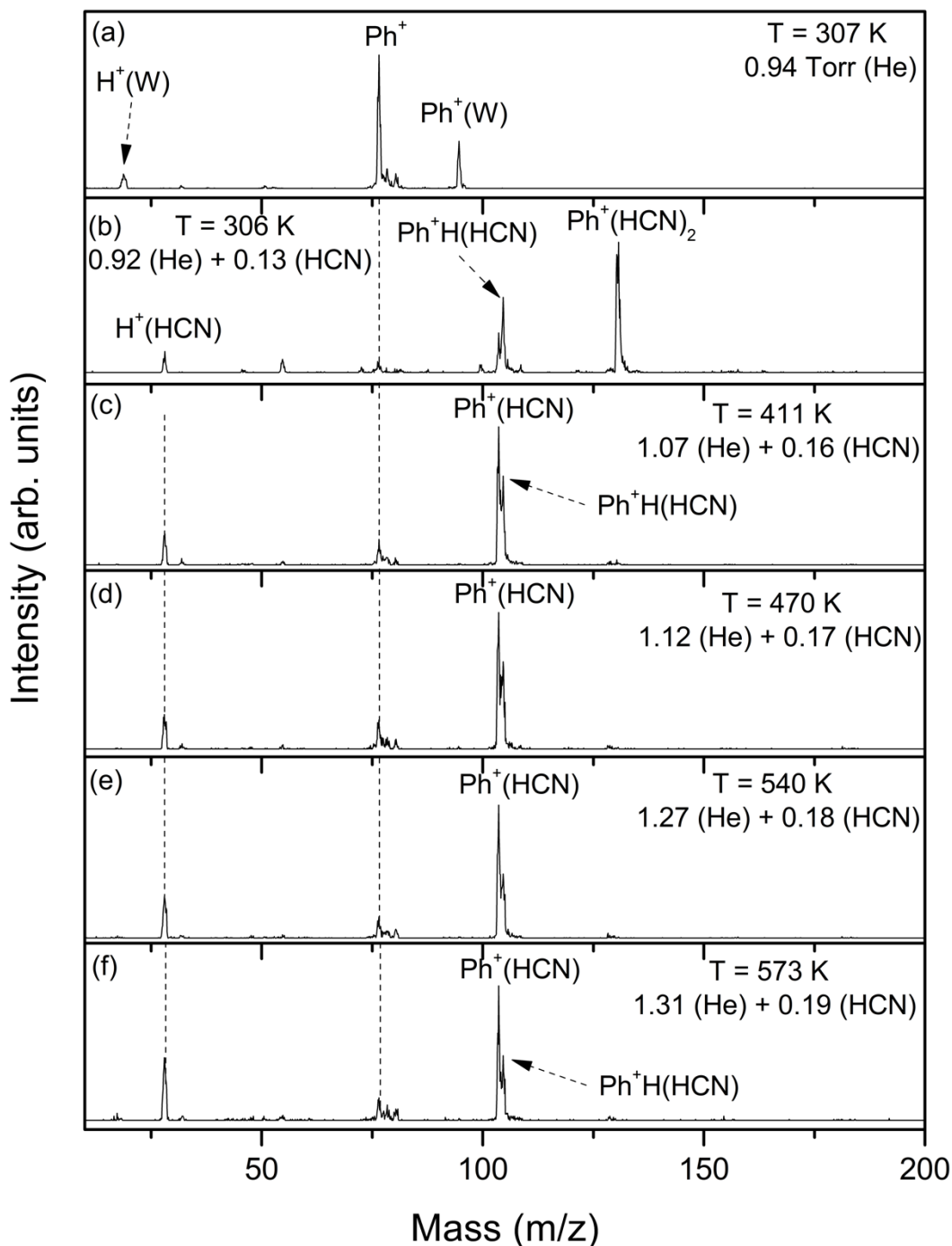
Figure 91. Mass spectra resulting from the injection of the mass-selected phenyl cations ( \text{C}_6\text{H}_5^+ , \text{Ph}^+ ) into He gas (a) or He/HCN gas mixture (b-f) at different pressures (Torr) and increasing temperatures (K) as indicated.
