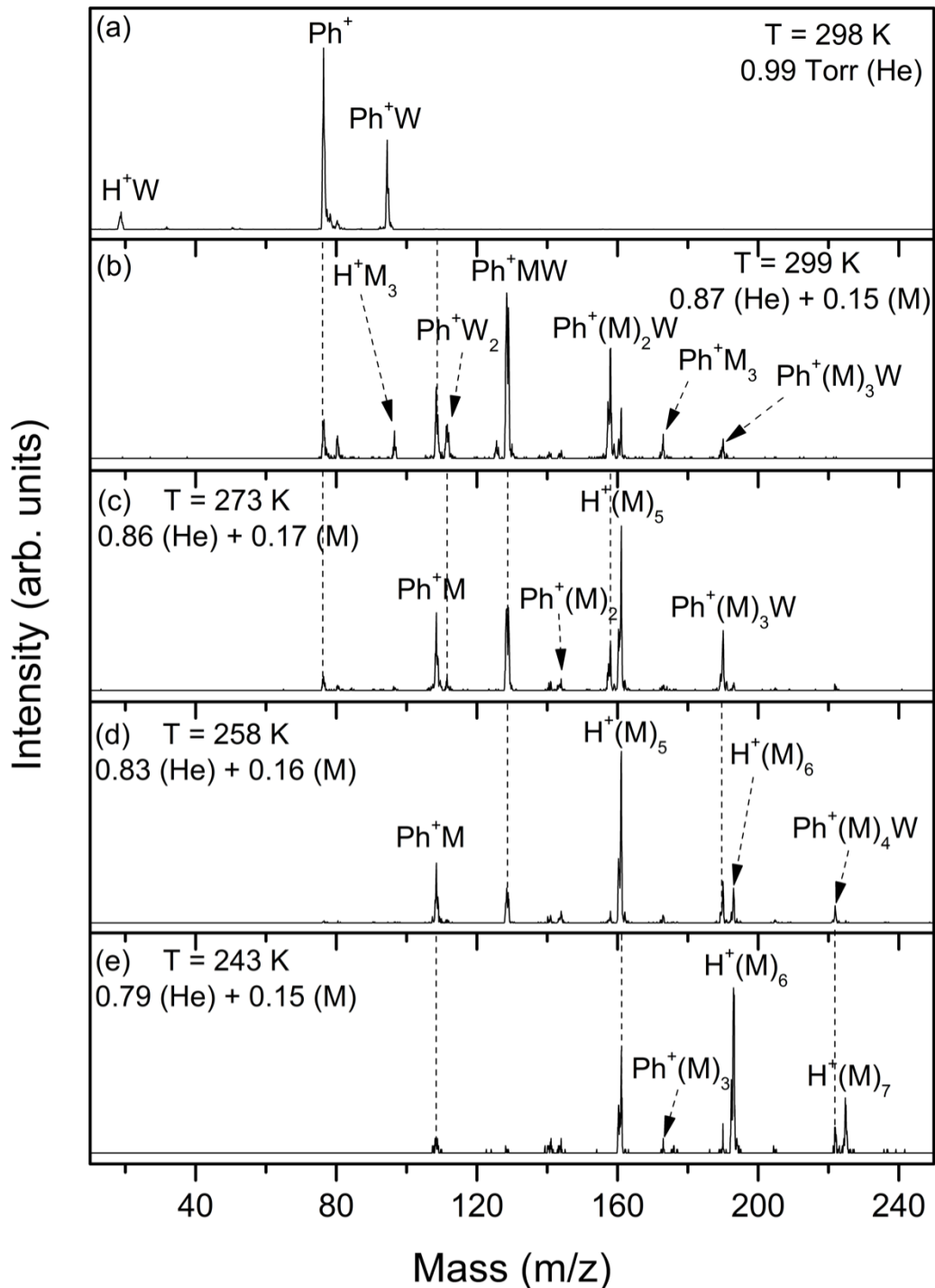
Figure 90. Mass spectra resulting from the injection of the mass-selected phenyl cation ( C_6H_5^+ , Ph^+ ) into He gas (a) or He/methanol (M) vapor mixture (b-e) at different pressures (Torr) and decreasing temperatures (K) as indicated.
