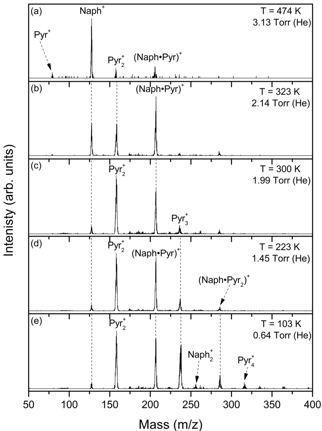
Figure 77. Mass spectra of the products of the coexpansion of a mixture of naphthalene and pyridine into the drift cell containing helium at the temperatures and pressures indicated. The ions are formed by 70 eV EI ionization and He was used as as carrier gas.
