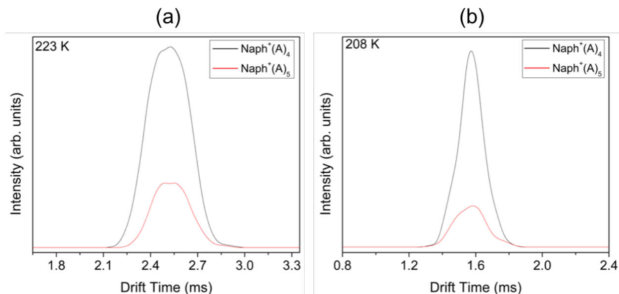
Figure 46. Arrival time distributions (ATDs) of the fourth and fifth association products of the naphthalene radical cation with acetonitrile (A), C_{10}H_8^{*+}(CH_3CN)_n for n = 4 and 5 ( Naph^+(A)_n n = 4, 5 ), obtained following the injection of the mass-selected naphthalene radical cation into the drift cell containing He/ CH_3CN vapor mixture at: (a) 223 K and (b) 208 K. Similar ATD overlap suggests the reaction is in equilibrium.
