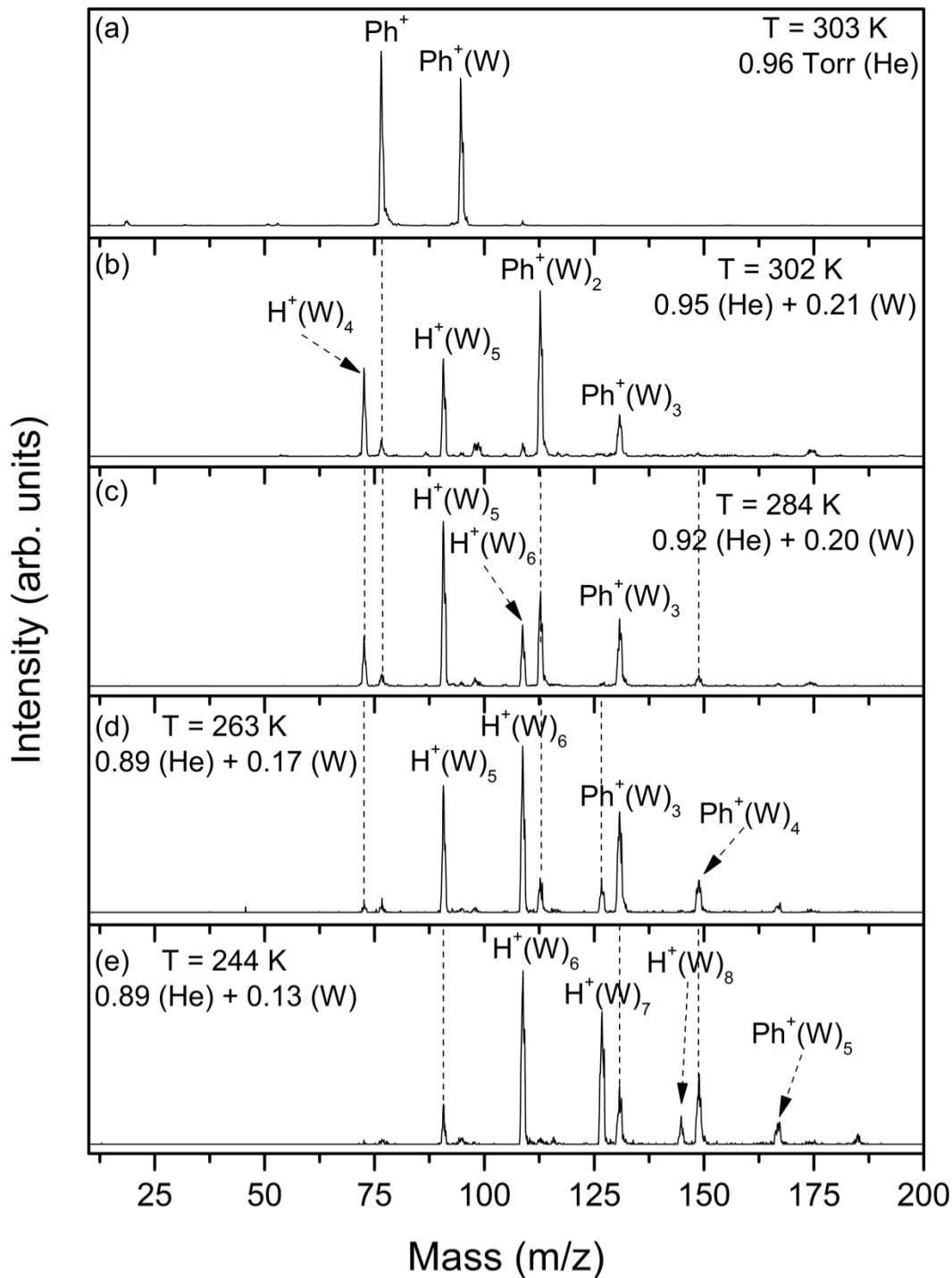
Figure 83. Mass spectra resulting from the injection of the mass-selected phenyl cation ( \text{C}_6\text{H}_5^+ , \text{Ph}^+ ) into He gas (a) or He/water (W) vapor mixture (b-e) at different pressures (Torr) and decreasing temperatures (K) as indicated.
