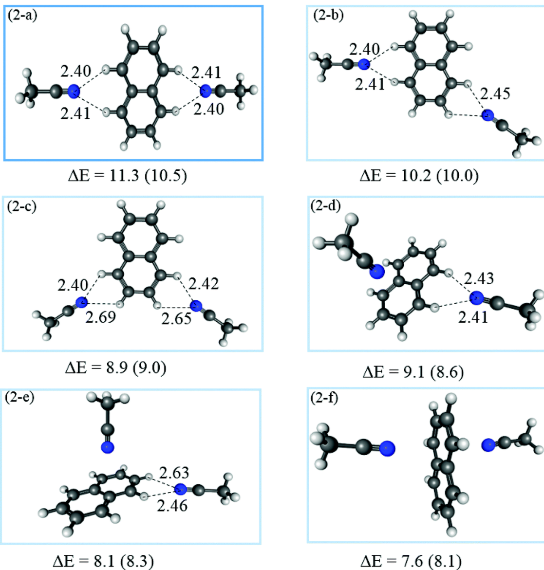
Figure 48. Structures of the six lowest energy isomers of the C_{10}H_8^+(CH_3CN)_2 complex obtained used two functionals: M06-2X and \omega 97X-D, within the 6-311+G** basis set. The calculated energies \Delta E in \text{kcal mol}^{-1} are given using M06-2X and \omega 97X-D (in parenthesis) methods.
