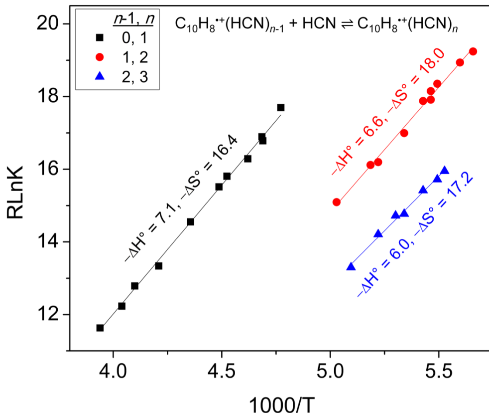
Figure 39. van't Hoff plots for the temperature dependence of the equilibrium constants of the association reaction of naphthalene radical cation with HCN for the first, second, and third solvation steps. The resulting \Delta H^\circ and \Delta S^\circ are in ( \text{kcal mol}^{-1} ) and ( \text{cal mol}^{-1} \text{K}^{-1} ) respectively. The experimental error for the -\Delta H^\circ and -\Delta S^\circ values are \pm 1 \text{ kcal mol}^{-1} and \pm 2 \text{ cal mol}^{-1} \text{K}^{-1} respectively.
