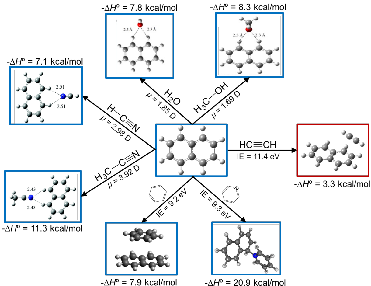
Figure 98. Summary of structures and binding energy (measured using -\Delta H^\circ with an experimental error of \pm 1 \text{ kcal mol}^{-1} ) for the first association product of the solvation of the naphthalene radical cation by various neutral molecules. Three classes are studied: (1) polar molecules ( \text{H}_2\text{O} , \text{CH}_3\text{OH} , \text{HCN} , and \text{CH}_3\text{CN} are shown), (2) unsaturated organic molecules (an estimate for \text{C}_2\text{H}_2 is shown), and (3) aromatic molecules ( \text{C}_6\text{H}_6 and \text{C}_5\text{H}_5\text{N} are shown). The structures were calculated at B3LYP/6-311++G** level for the polar molecules, M11/cc-pVTZ level for \text{C}_6\text{H}_6 , and M06-2X/cc-pVTZ level for \text{C}_5\text{H}_5\text{N} .
