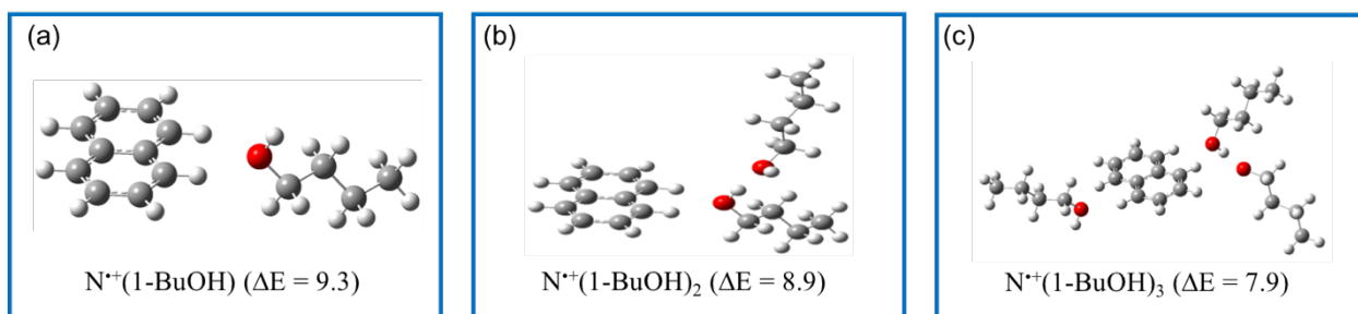
Figure 34. DFT structures and binding energies ( \Delta E kcal mol -1 , calculated according to Equation 4.3) of the lowest energy isomers of the C_{10}H_8^{+\cdot}(1-BuOH)_n clusters for n = 1-3 obtained at the B3LYP/6-311++G** level.
