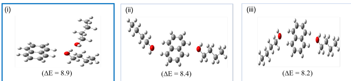
(c) C_{10}H_8^{*+}(1-BuOH)_3
