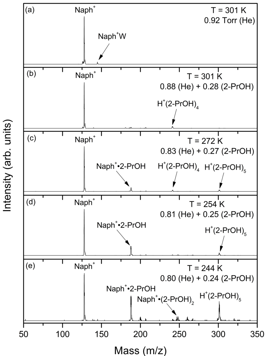
Figure 21. Mass spectra resulting from the injection of the mass-selected naphthalene radical cations ( C_{10}H_8^+ , Naph^+ ) into He gas (a) or He/2-propanol (2-PrOH) vapor mixture (b-e) at different pressures (Torr) and temperatures (K) as indicated.
