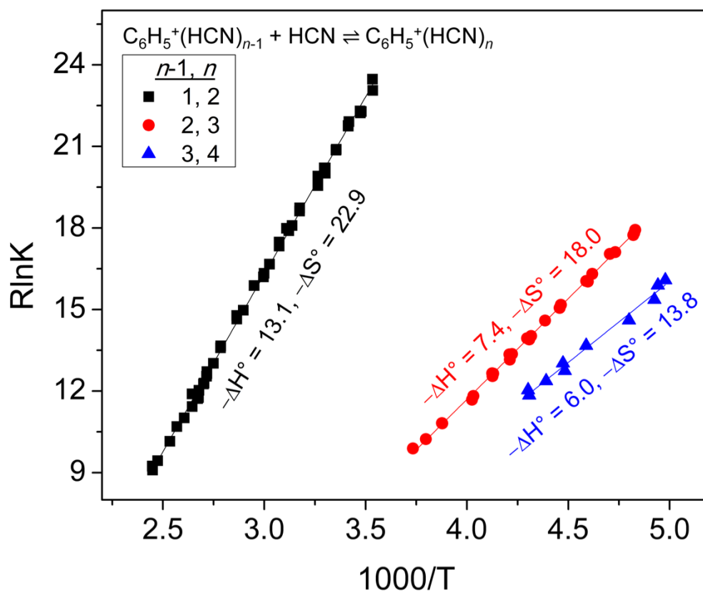
Figure 93. van't Hoff plot for the temperature dependence of the equilibrium constants of the association reaction of phenyl cation with HCN for the second, third, and fourth solvation products. The resulting -\Delta H^\circ and -\Delta S^\circ are in ( \text{kcal mol}^{-1} ) and ( \text{cal mol}^{-1} \text{ K}^{-1} ) respectively. The experimental error for these measurements are \pm 1 \text{ kcal mol}^{-1} and \pm 2 \text{ cal mol}^{-1} \text{ K}^{-1} .
