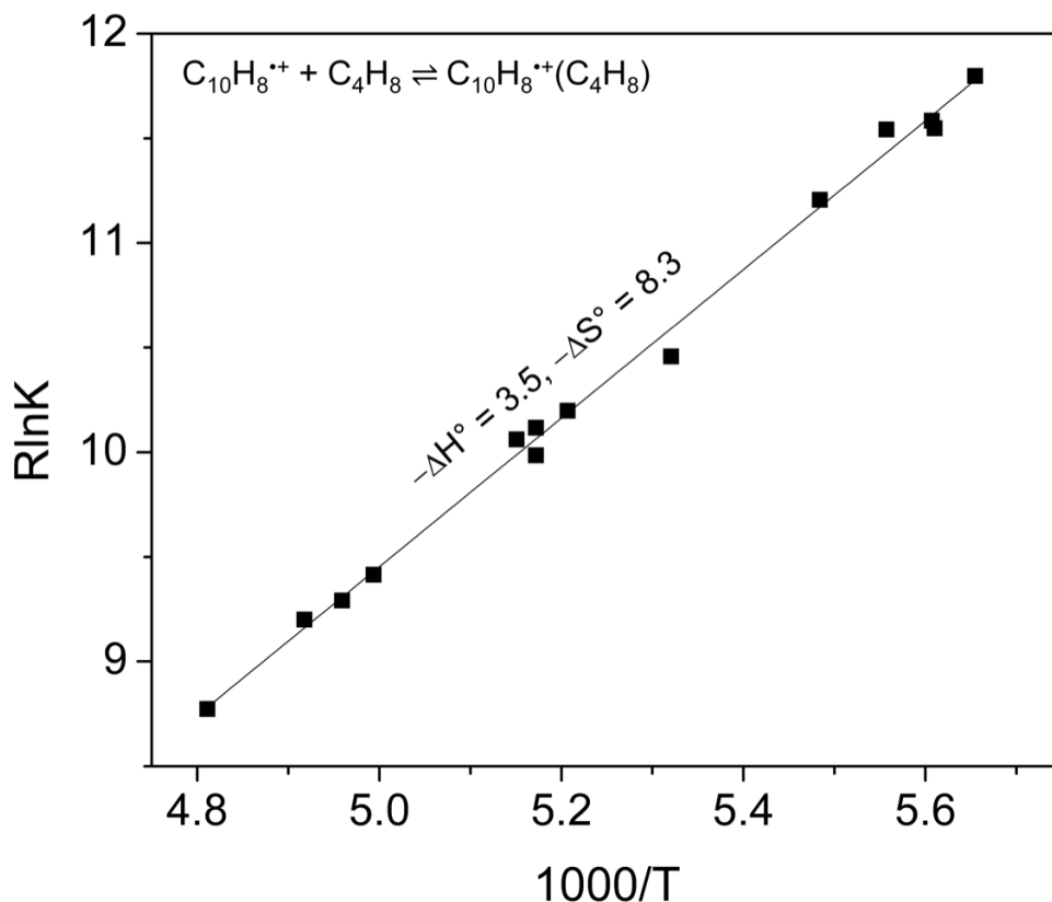
Figure 60. van't Hoff plot for the temperature dependence of the equilibrium constants of the association reaction of naphthalene radical cation with isobutene for the first step. The resulting \Delta H^\circ and \Delta S^\circ are in ( \text{kcal mol}^{-1} ) and ( \text{cal mol}^{-1} \text{K}^{-1} ) respectively. The error for the measurements are \pm 1 \text{ kcal mol}^{-1} for -\Delta H^\circ and \pm 2 \text{ cal mol}^{-1} \text{K}^{-1} for -\Delta S^\circ .
